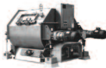
Stainless Food Grade Batch Mixer on Load Cells To 600 cu. ft. Cv 5% in 30 seconds
